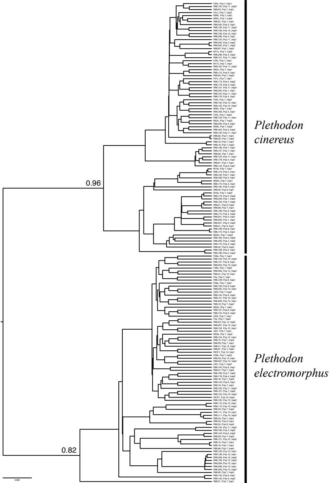
Supplemental Fig. 1. POMC gene tree inferred using *BEAST 2. Tip labels include collector number, followed by sample locality (Table 1, Fig. 1) and haplotype number (1 or 2). The species to which each clade applies is labeled at the right, and the posterior probability of these clades is provided above the relevant nodes.
